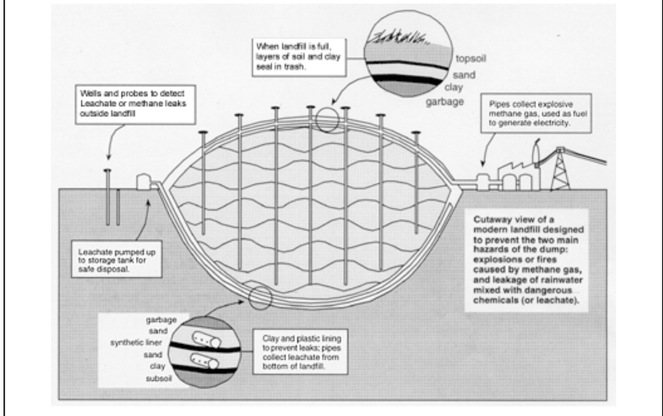
Figure II-4: Cross-Section of a Municipal Solid Waste Landfill
